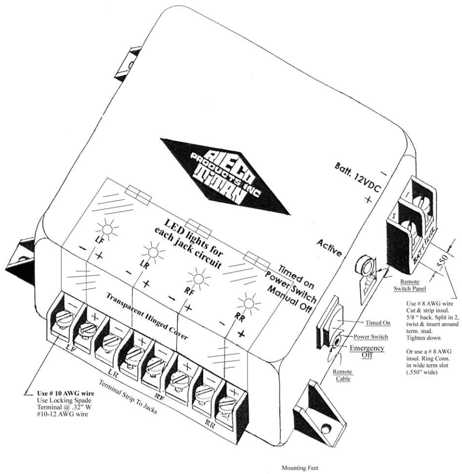
WIRED-WIRELESS RECEIVER CONTROL BOX
