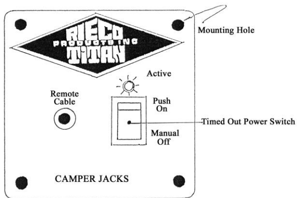
REMOTE SWITCH PANEL
